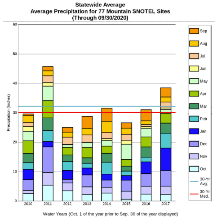
Image 3: Statewide Average- Average Precipitation
