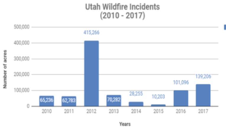
Image 2: Utah Wildfire Incidents (2010-2017).
