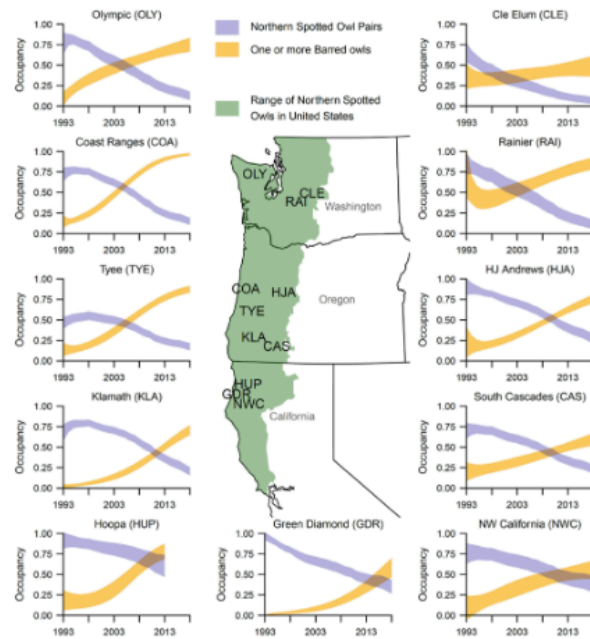
Diagram 3: Trends in territory occupancy for northern spotted owl pairs and barred owls on 11 study areas in Washington, Oregon, and California based on two-species occupancy models from 1993–2018
