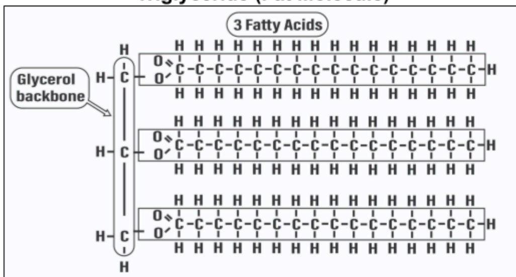
Triglyceride (Fat Molecule)
