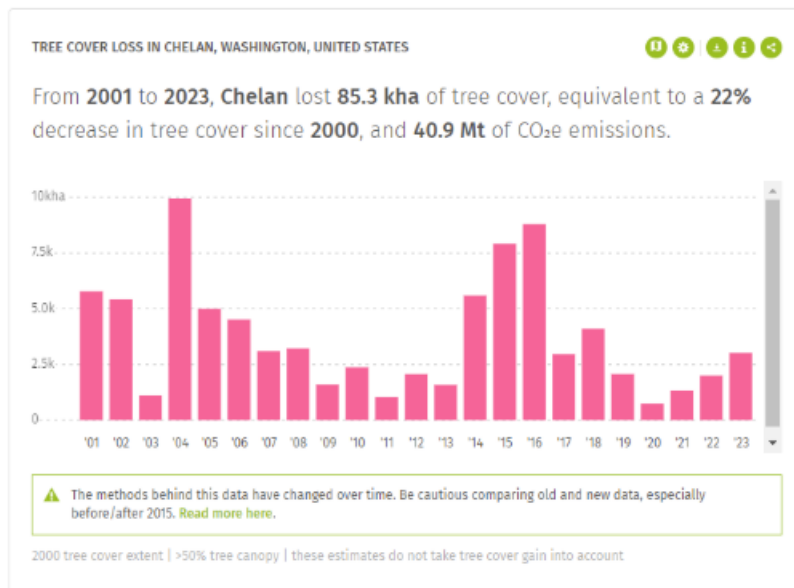
Diagram 4: Tree Cover Loss in Chelan, Washington, United States
