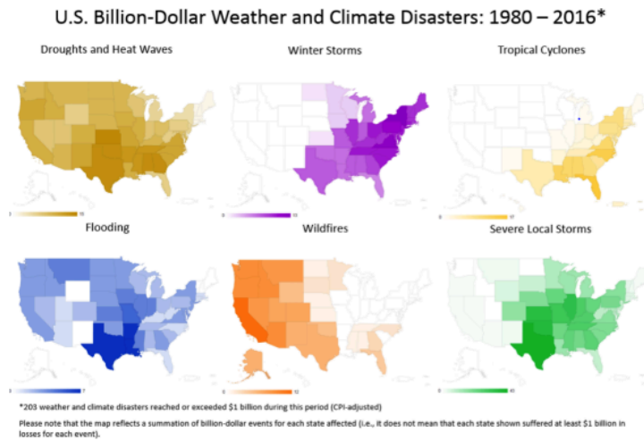
Image 1: U.S. Billion-Dollar Weather and Climate Disasters: 1980-2016
